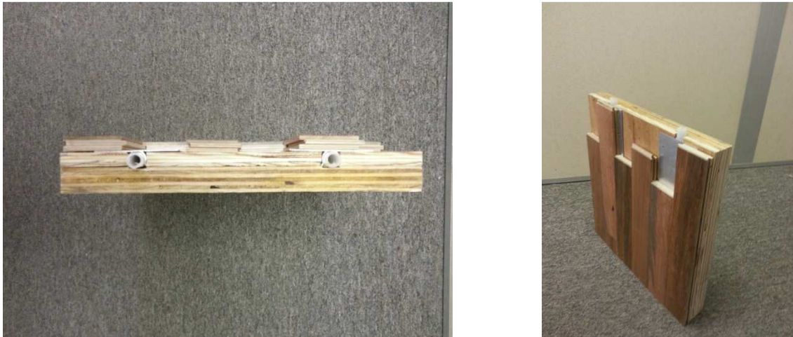
Figure 5. Floor Sections
